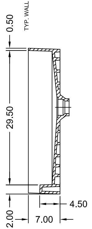
SECTION B-B
