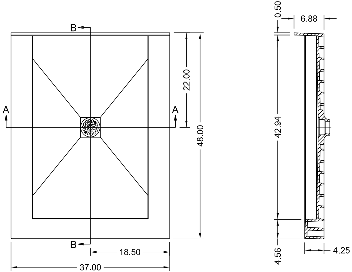
SECTION B-B
