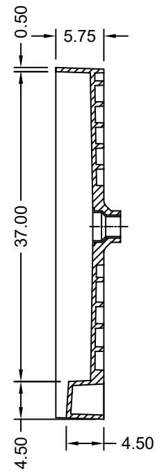
SECTION B-B
