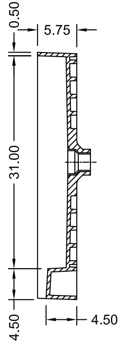
SECTION B-B
