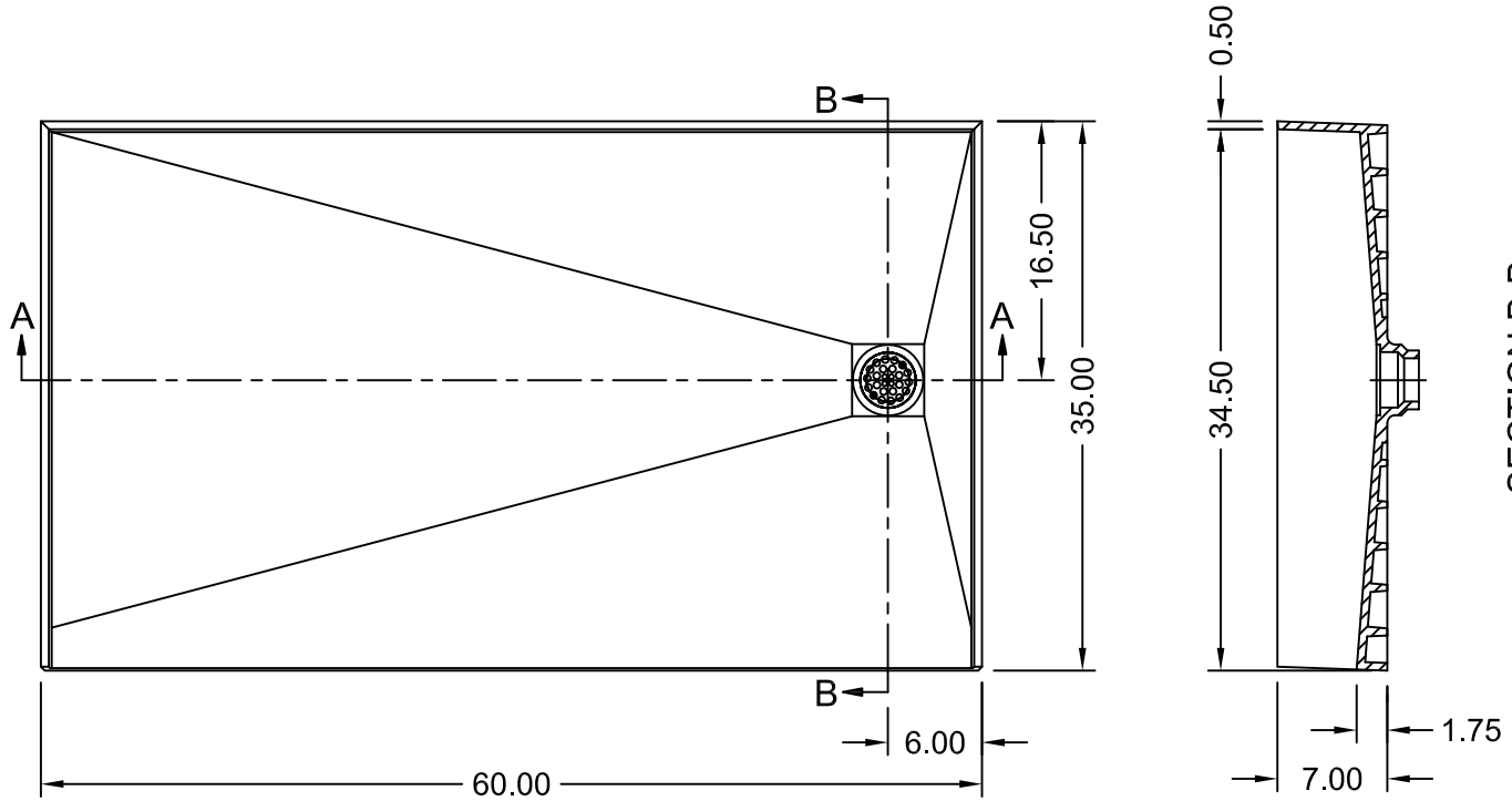
SECTION B-B
