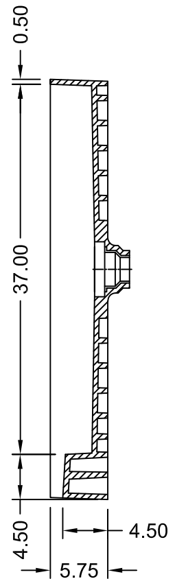
SECTION B-B
