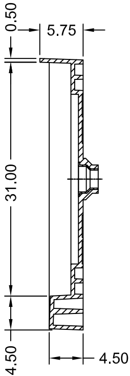
SECTION B-B
