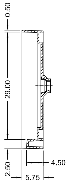
SECTION B-B
