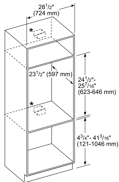
Single Steam Oven Wall mount installation
