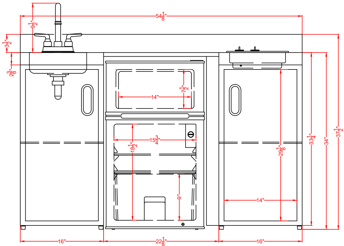
FRONT VIEW
