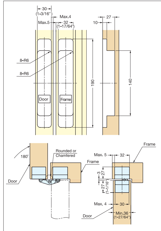
Bore Dimensions
