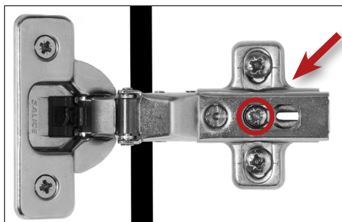
Adjusting door in & out
