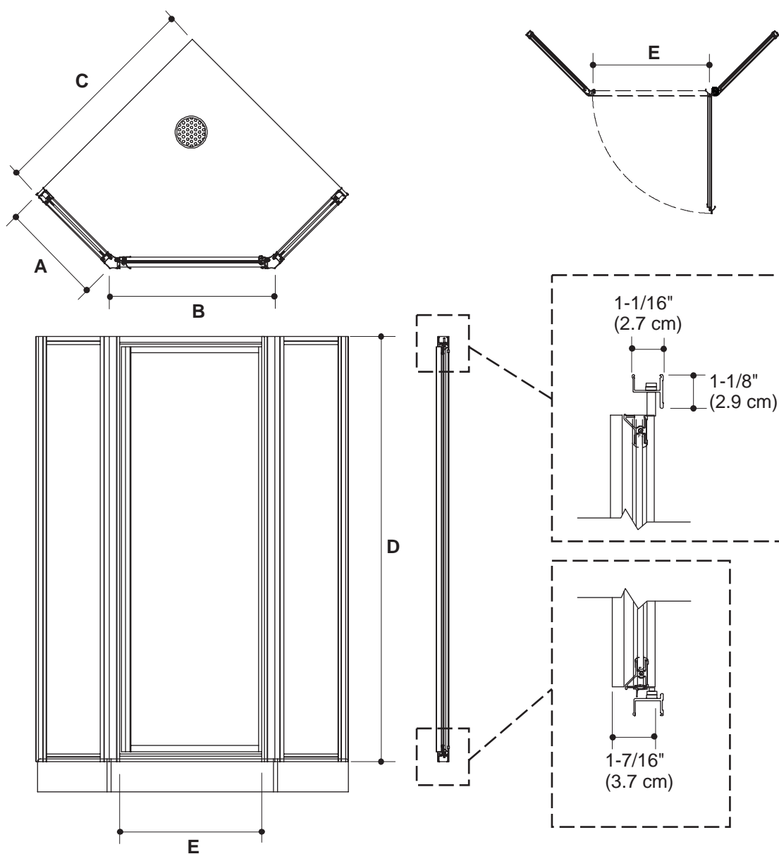
Product Diagram
