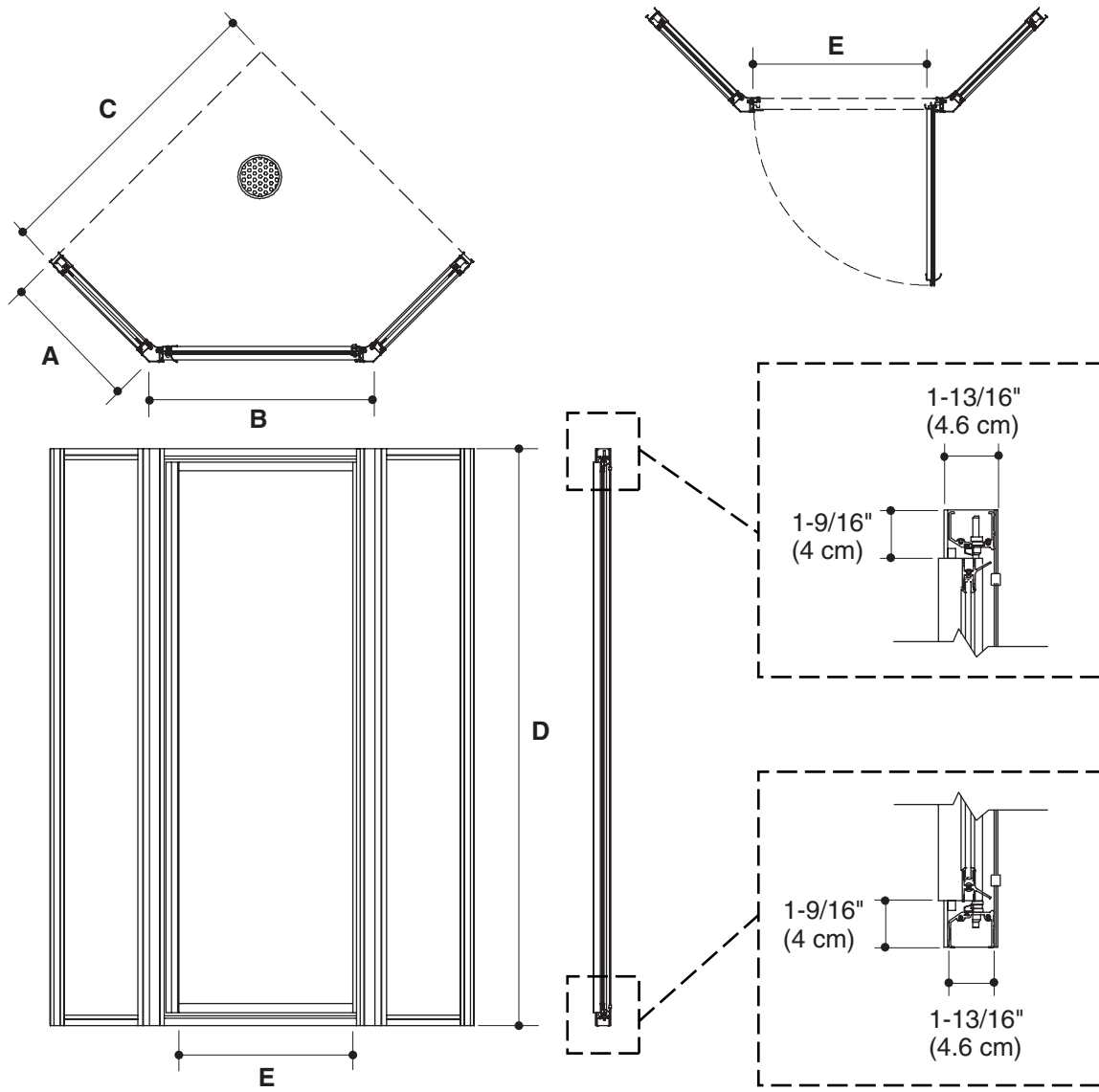
Product Diagram
