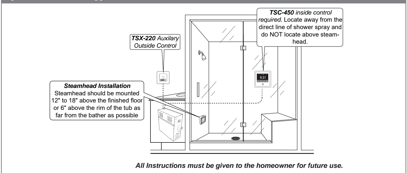
Figure 5 - Installation Suggestions
