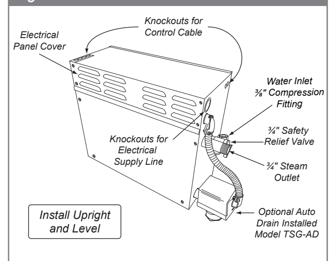
Figure 1- Steam Generator
