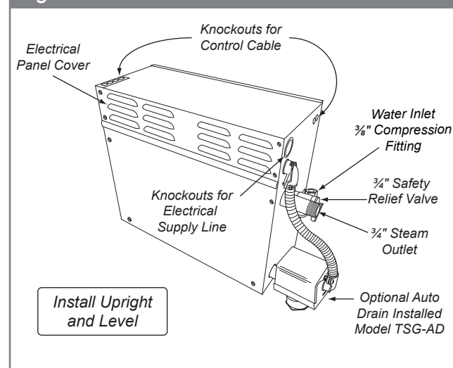
Figure 1- Steam Generator
