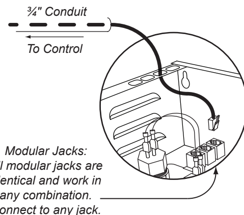
Figure 3 - Cable Installation on Steam Generator
