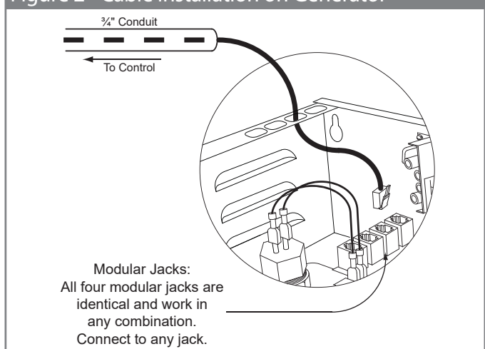
Figure 2 - Cable Installation on Generator
