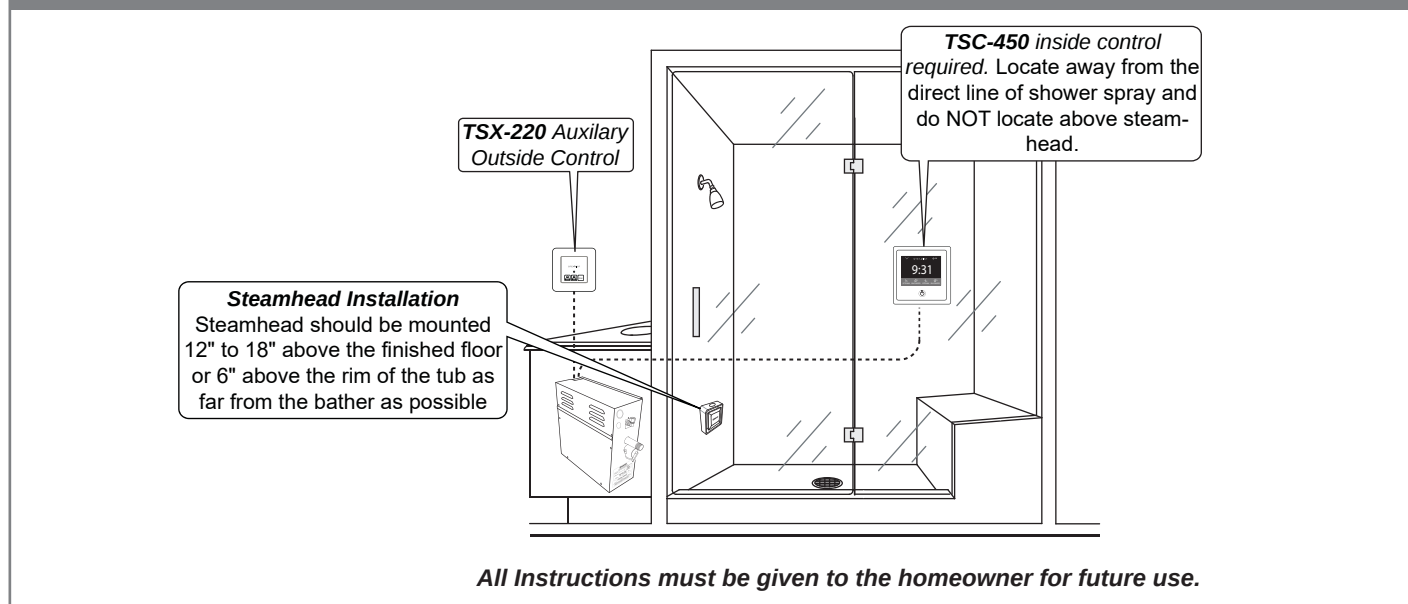
Figure 5 - Installation Suggestions
