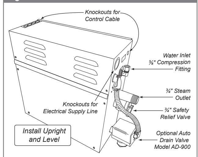
Figure 1 - Steam Generator
