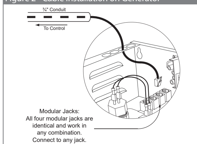
Figure 2 - Cable Installation on Generator
