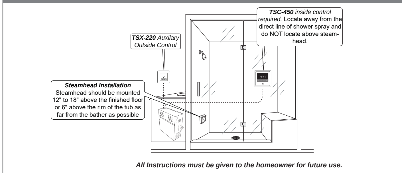
Figure 5 - Installation Suggestions
