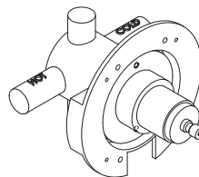
KOHLER® Rite-Temp®
