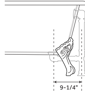
Optional Overflow Rough-in
