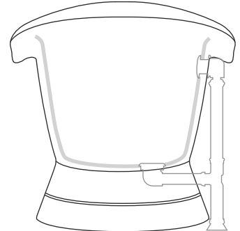
Optional Overflow Rough-in
