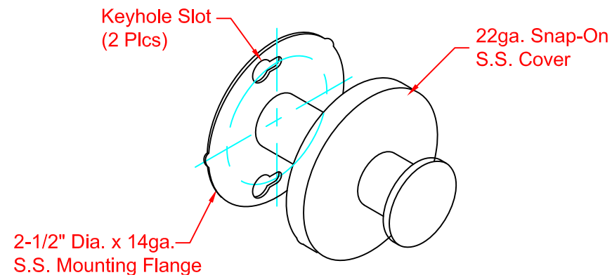
Mounting Flange Detail
