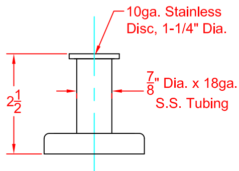
ASSEMBLY VIEW
