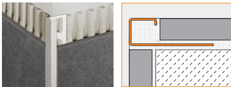
2.10 Schluter®-QUADEC
