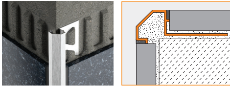
2.13 Schluter®-DIADEC
