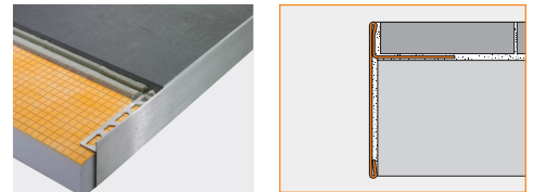
2.11 Schluter®-SCHIENE-STEP
