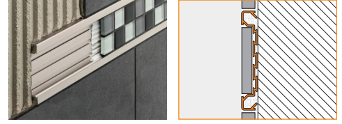
2.11 Schluter®-QUADEC-FS
