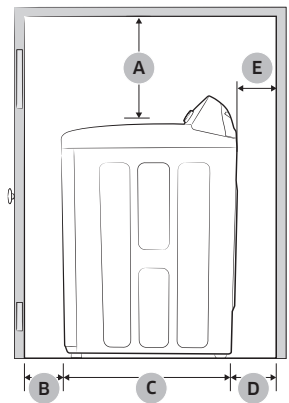
Side view - closet or confined area
