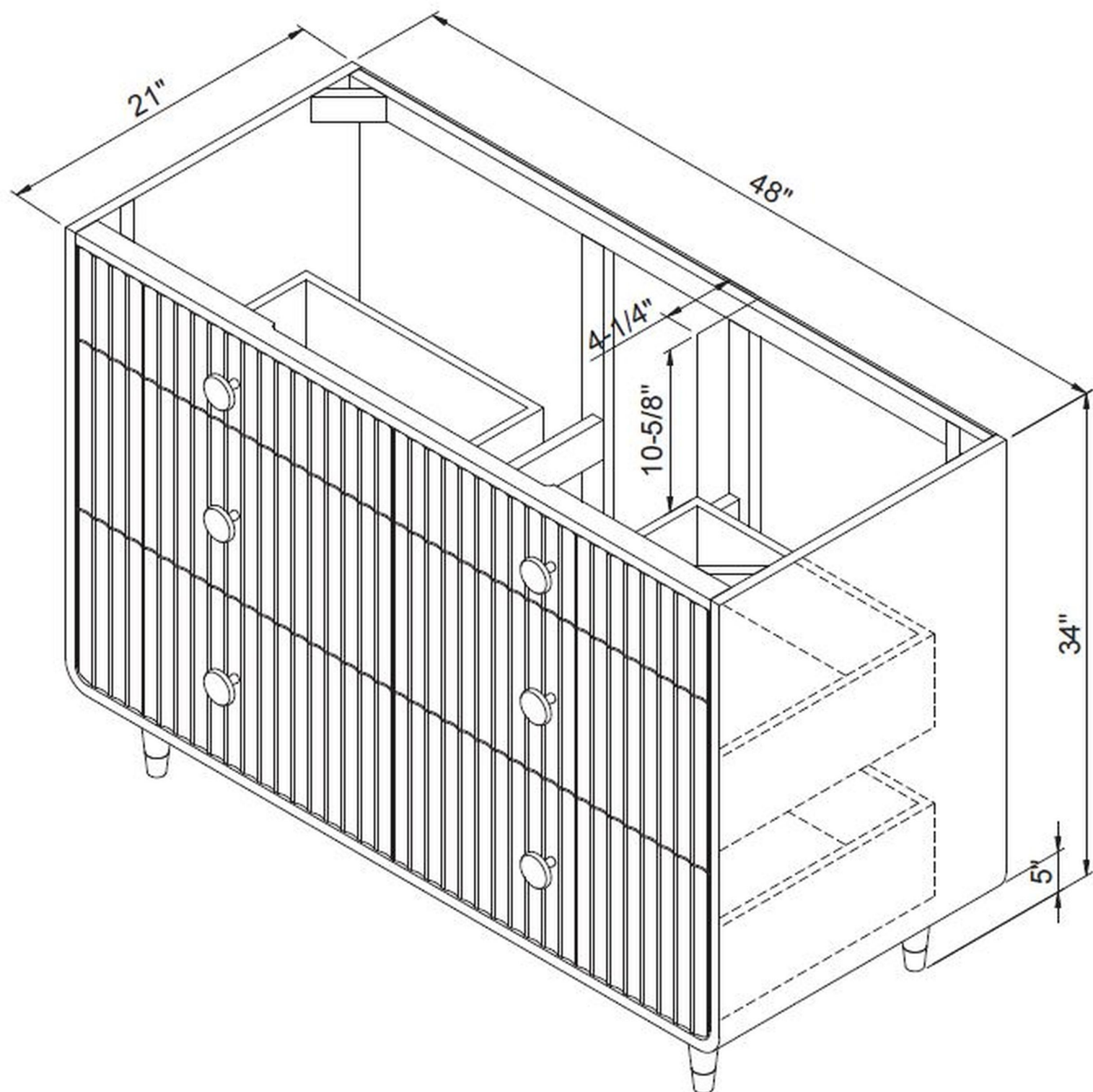
KB4821D Vanity 4 x Drawer
