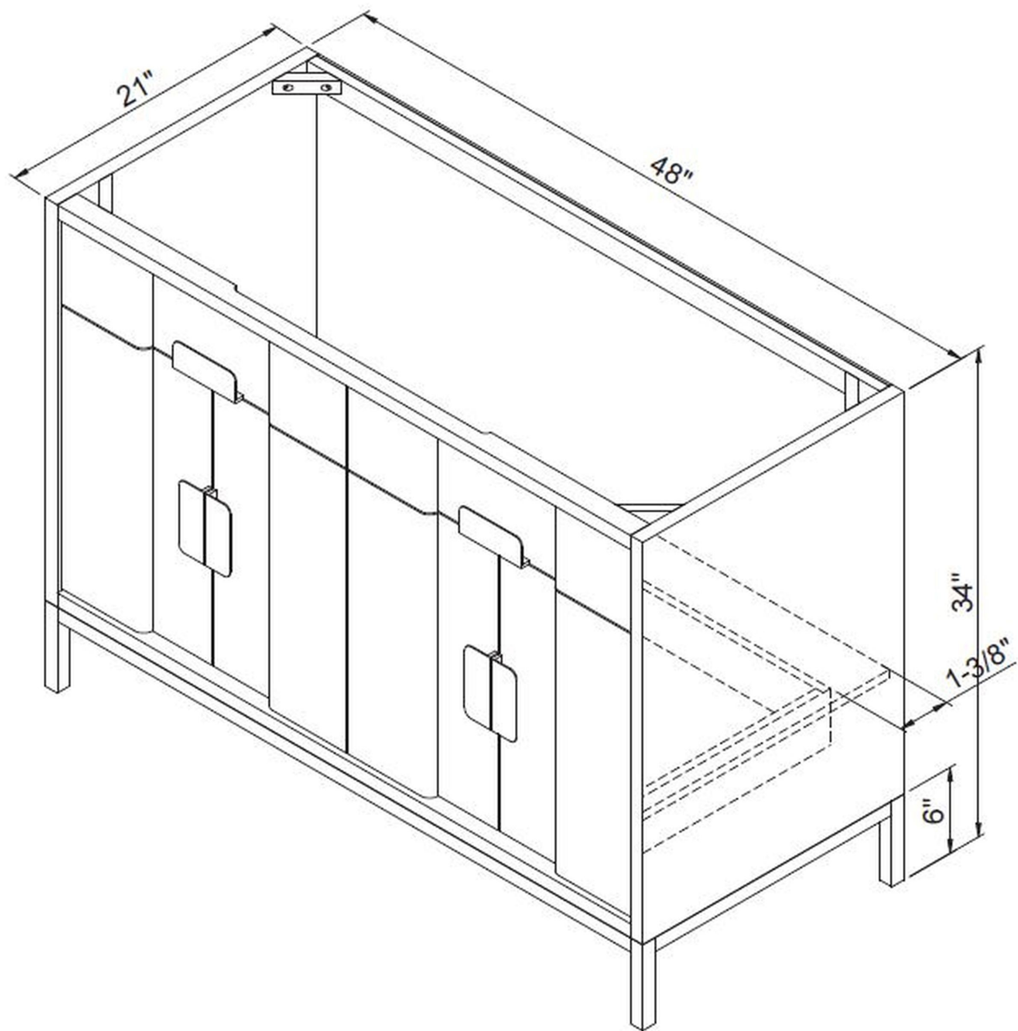
IL4821D Vanity 2 x Drawer
