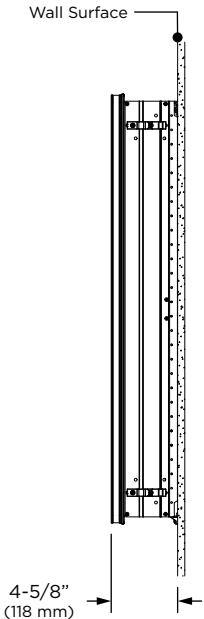
Surface Mount
