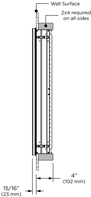
Recessed Mount
