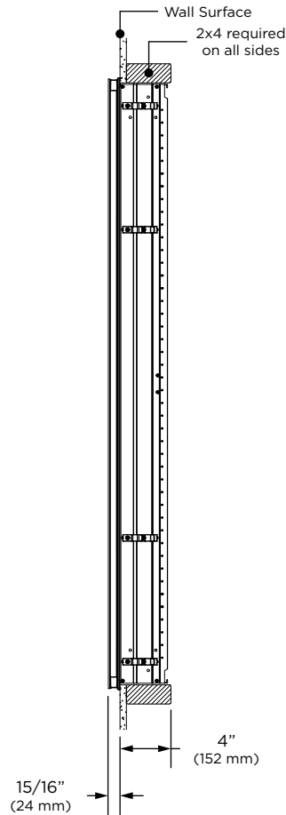
Recessed Mount
