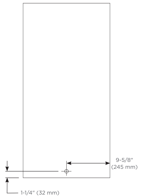
Back of Cabinet - Wire Access Location
