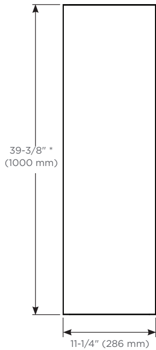
Cabinet Dimensions
