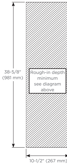
Rough-in Dimensions
