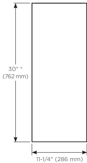
Cabinet Dimensions
