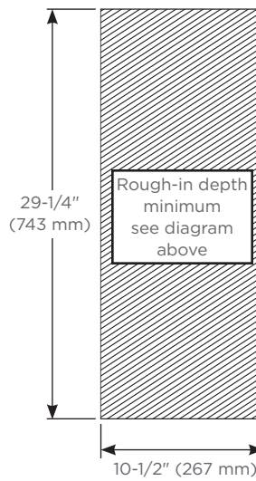
Rough-in Dimensions
