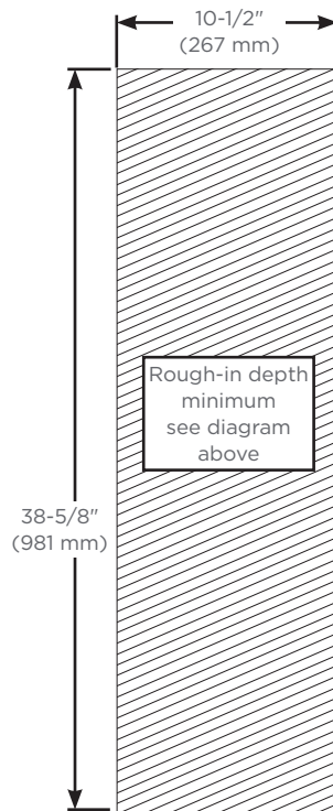
Rough-in Dimensions Recessed mount only
