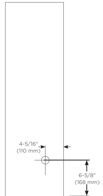
Back of Cabinet - Wire Access Location
