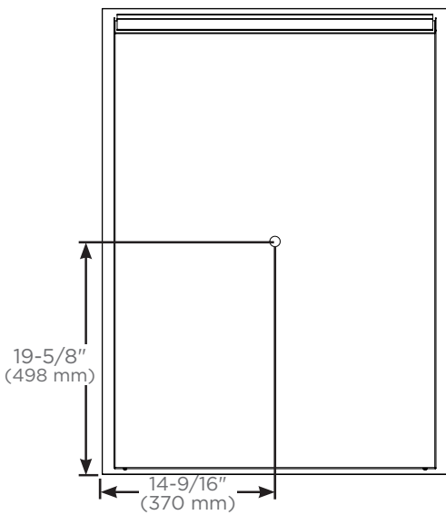
Back view for electrical knockout location
