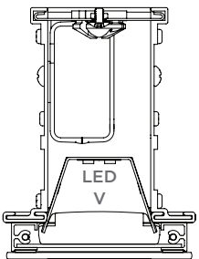
Cross Section
