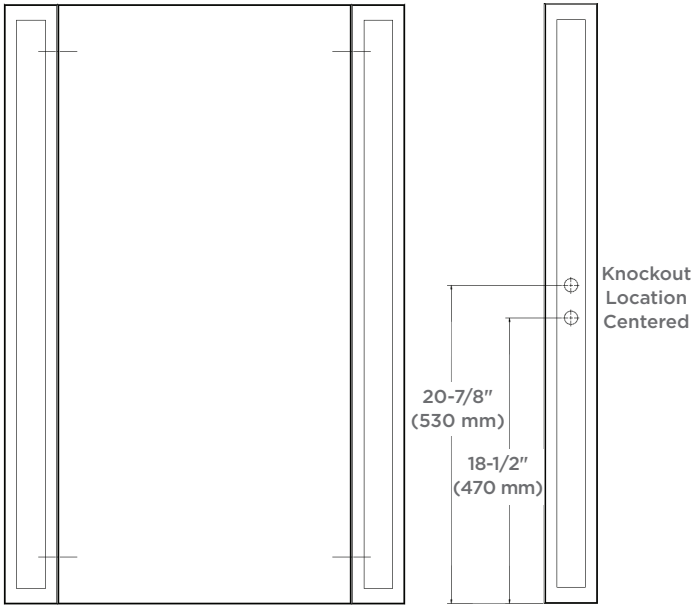
Typical Ganged Arrangement
