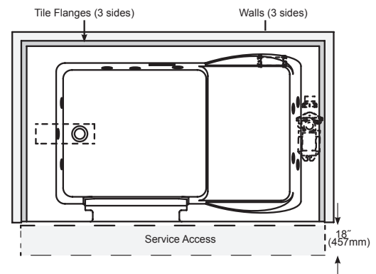
5230/6030 Walk-In Bathtub
