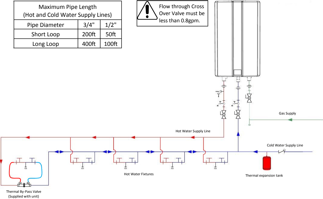
Cross Over Method Plumbing Diagram
