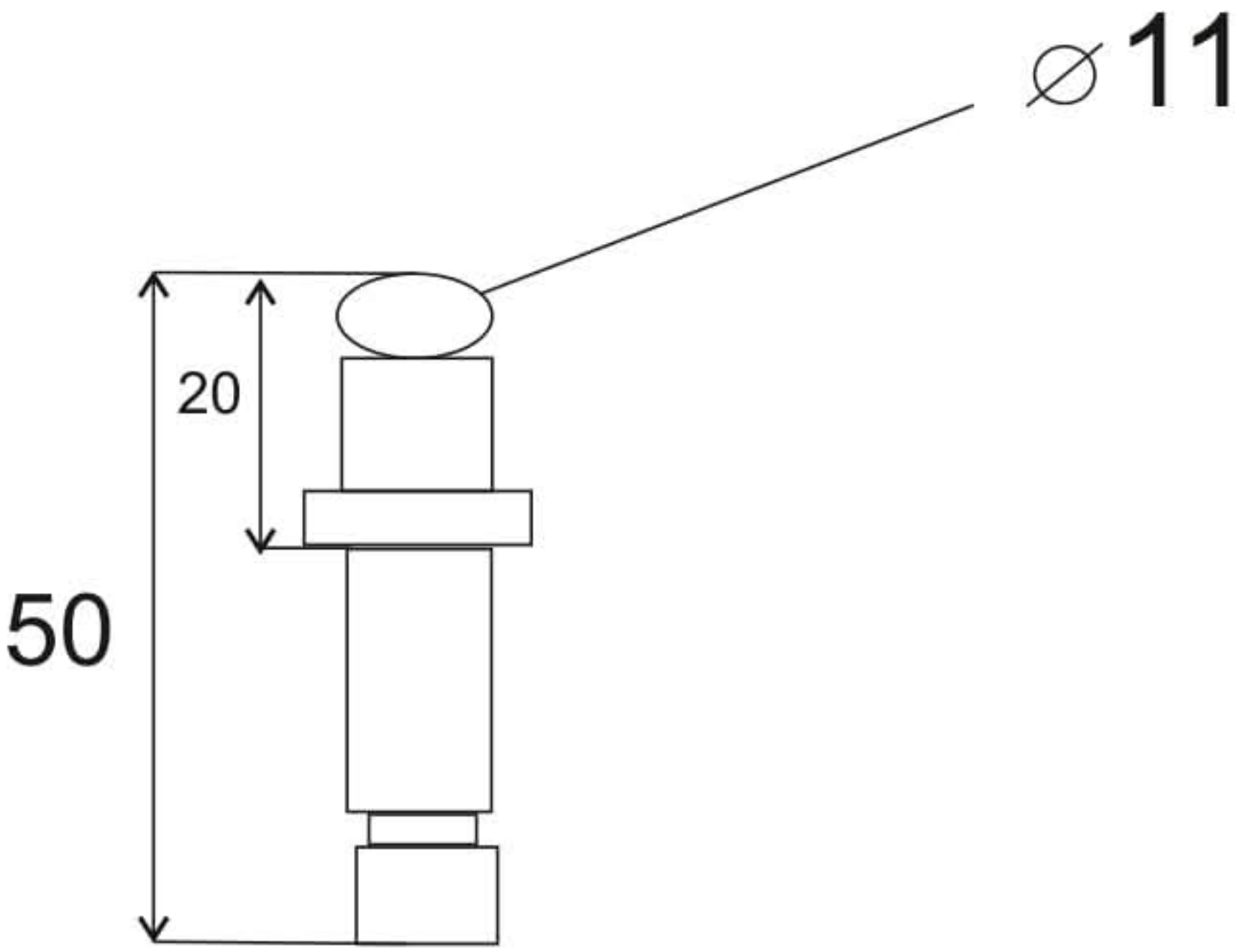
11x20 pin attachment
