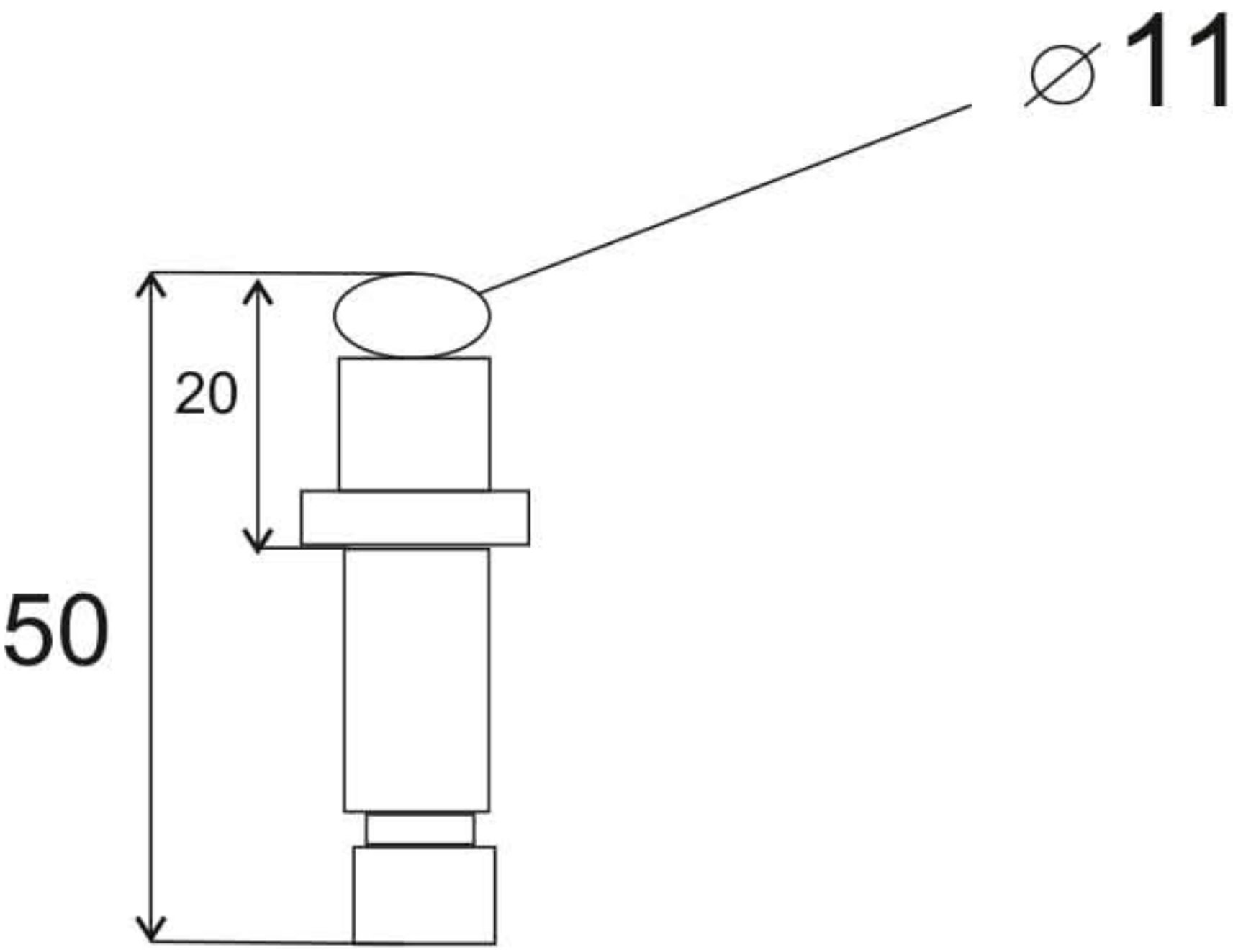
11x20 pin attachment
