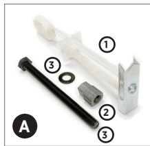
Drywall Anchor with Bolt, Washer & Plug (1) BD17-BD200-009 (2) BD17-BD200-007 (3) BD134-MB
