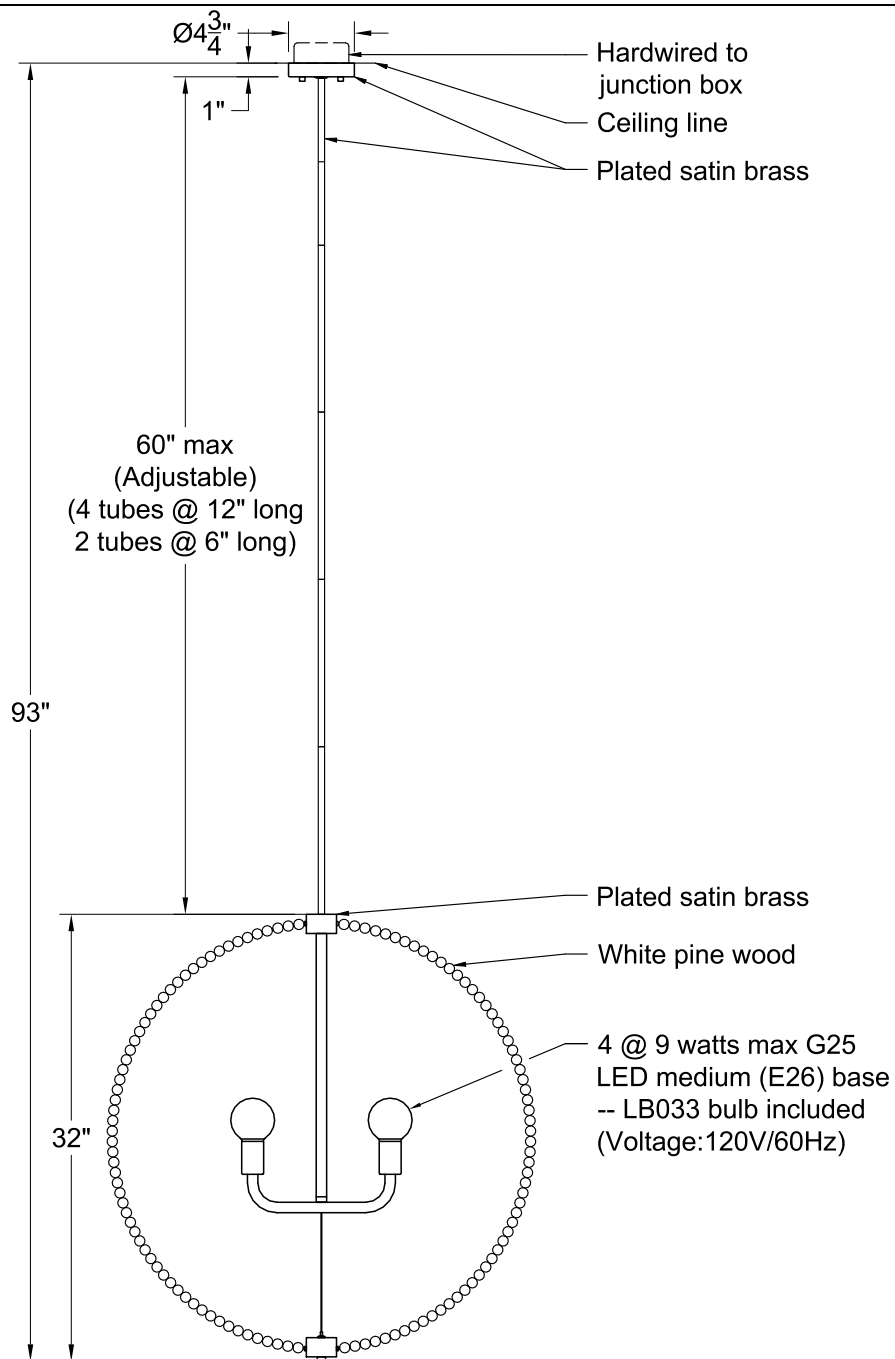
FRONT VIEW
