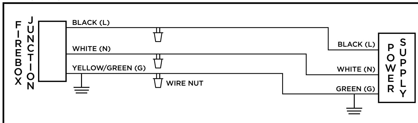
Wiring Diagram
