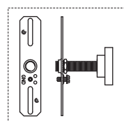
A Crossbar Assembly x 1
