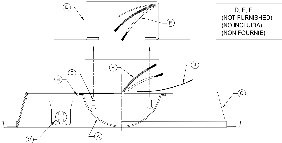
DETAIL "A"/DETALLE "A"/DÉTAIL "A"
