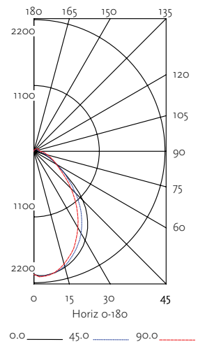
Test 15387 Test Date 7/18/14 INDOOR CANDELA PLOT
