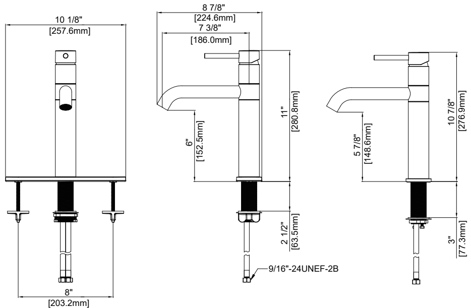
With Escutcheon
