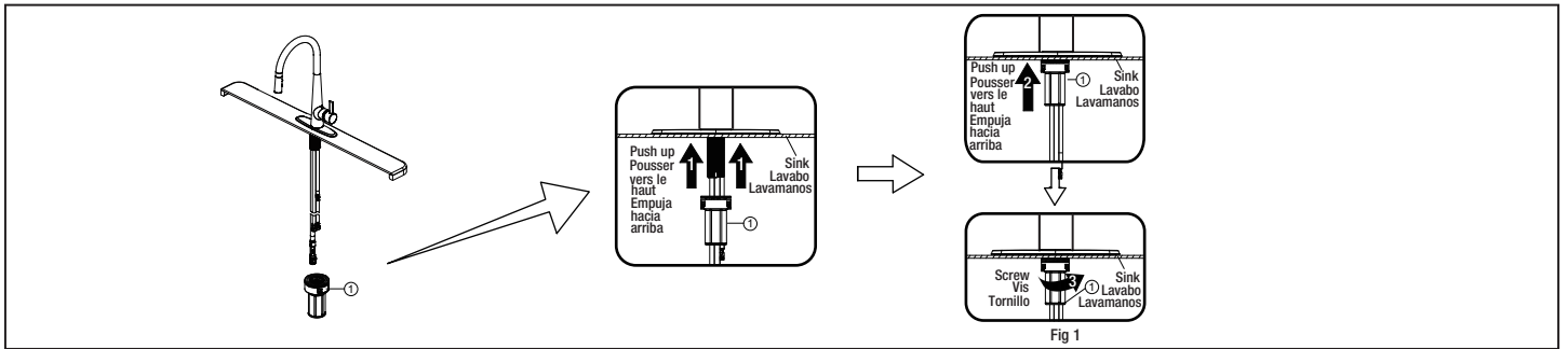
2. From underneath the sink, secure the faucet assembly to the sink with the quick install nut (1). Push the quick install nut (1) up over the threads until it stops against the bottom of the sink, then hand turn (clockwise) to tighten (Fig 1).
