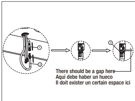
3. Connect the outlet hose (1) with pull-down hose (2). Confirm the bushing (3) return to original state.
