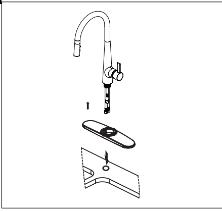
1. Install the escutcheon on the faucet. Place new faucet through holes in top of sink.
