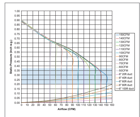
FV-15NLF51 50-150 CFM 6" Duct
