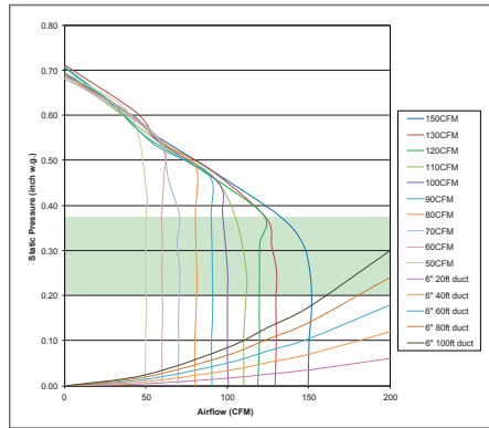
FV-1115VKL2 50-80-110 CFM 4" or 6" Duct
