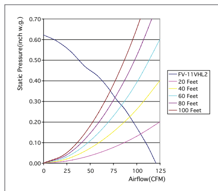
FV-11VHL2 110 CFM 4" Duct
