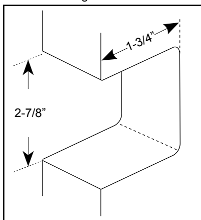
Notching Dimensions
