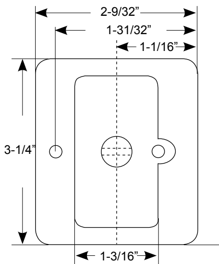
Notching Dimensions
